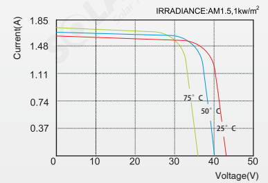
SLP050-24U I-V Curves
